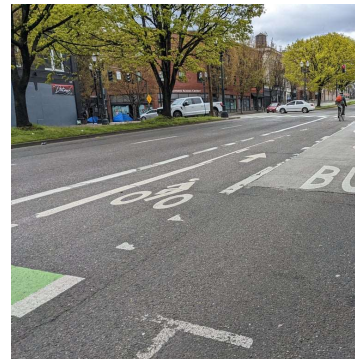
Class II Buffered Bike Lane
