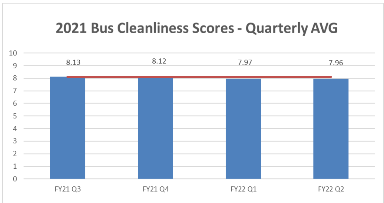
Chart 2 – BCI Scores
