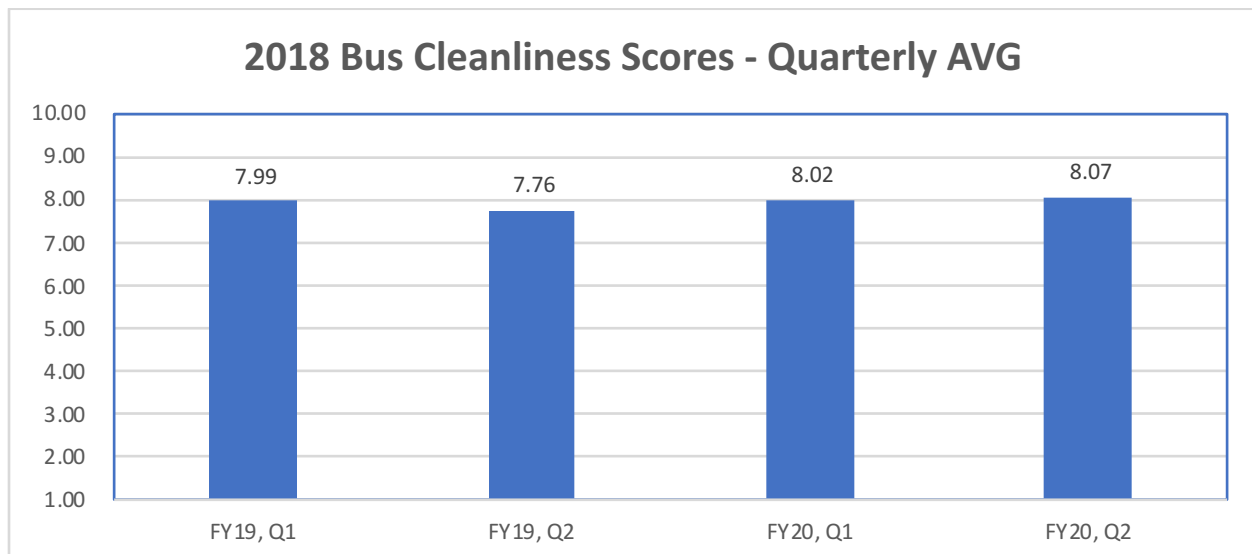
Chart 2 – BCI Scores
